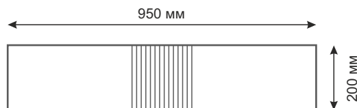
DECORATIVE PANEL #1 MDF, COPLANAR for Duo-408 (950x200x10 mm)
